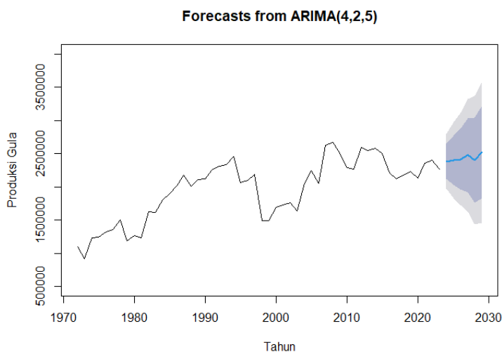
Gambar 6.2. Plot Hasil Ramalan Model ARIMA (4,2,5)
