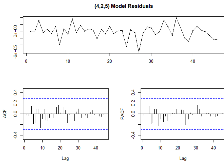
Gambar 6.1. Plot Sisaan Model ARIMA (4,2,5)
